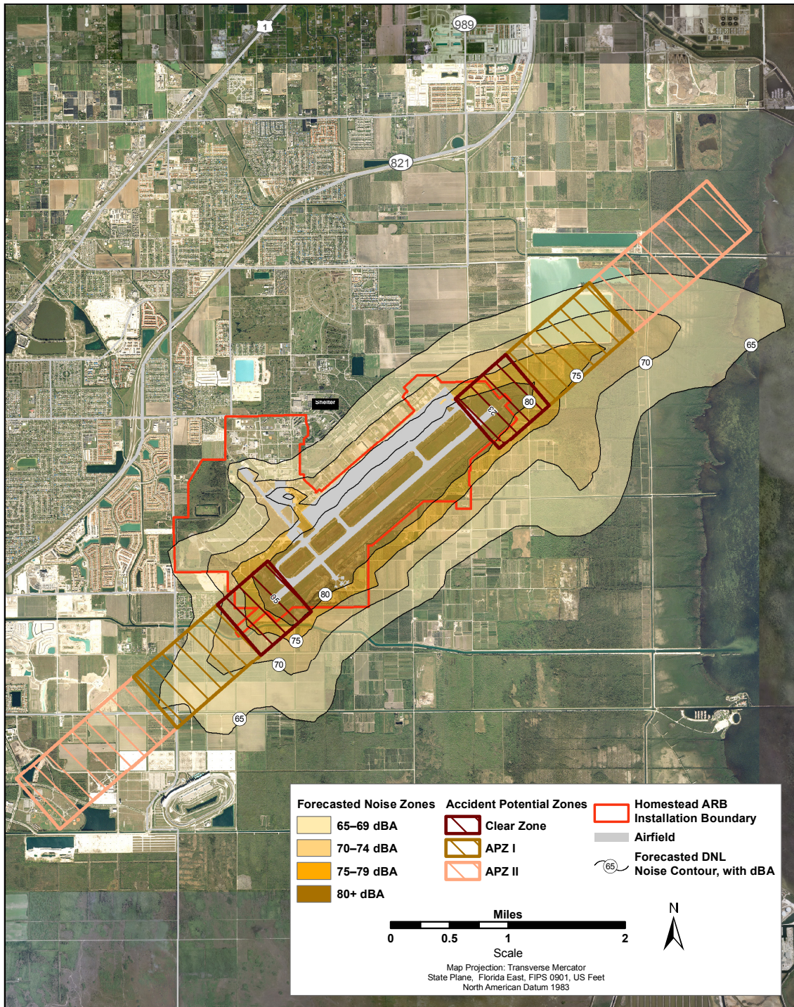
Figure 3-1. Accident Potential Zones and Forecasted Noise Zones
